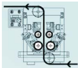
Water Wash Traversing Web Cleaner
